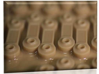
3D Printing
